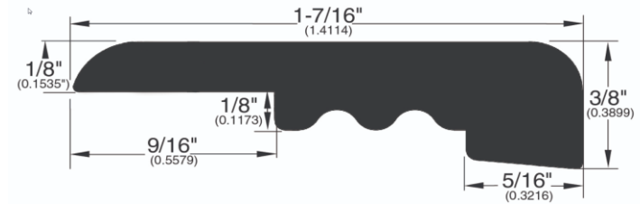
Square Nose (281004)
