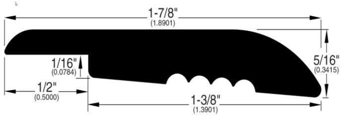
Overlap Reducer (280990)
