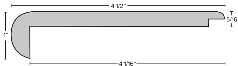
Flush Stair Nose: combine with Durato SPC flooring to cover stair treads. 94.5" Long.
